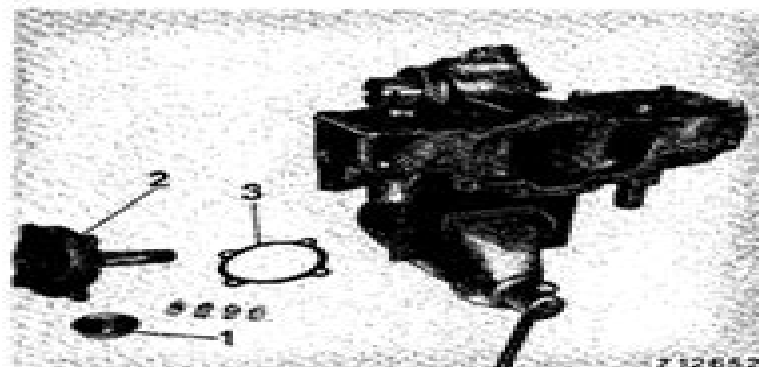
Fig. 5 — Removing Gatherer Cap, Shaft and End Cap
