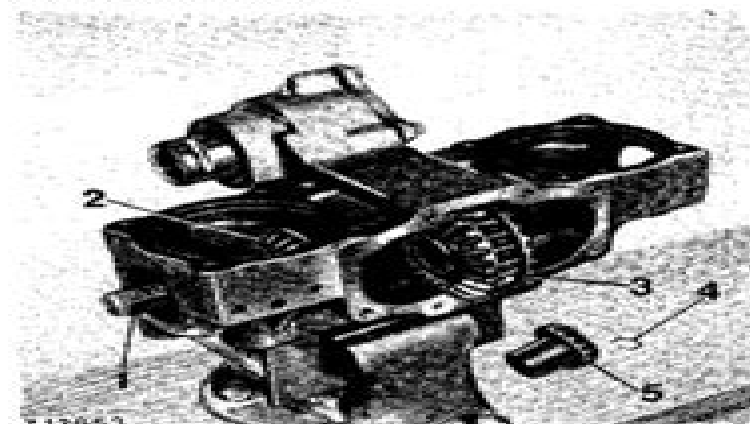
Fig. 6 — Removing Hex. Countershaft, Bevel Gears and Gear Cluster
