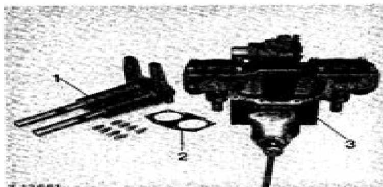
Fig. 4 — Disassembling Gear Case
