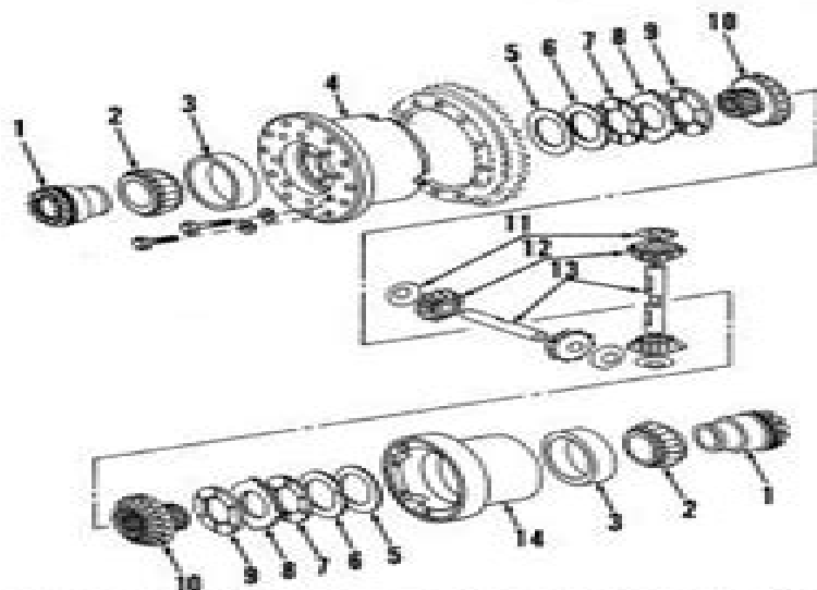
Fig. 282—Exploded view of differential assembly. Note that thick friction disc (9) is installed next to side gear (10) with friction facing towards separator plate (8). Shims (5) are installed between last separator plate and differential case.
