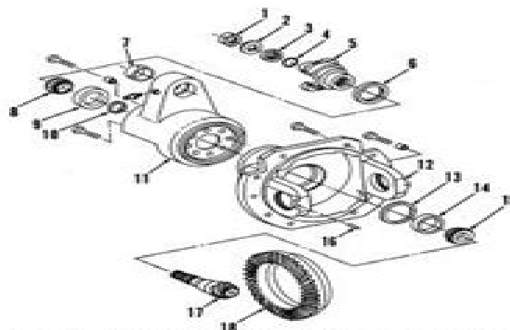
Fig. 283—Exploded view of bevel ring gear and pinion and associated components. Pinion shaft cone point is adjusted by shims (13). Pinion shaft bearings are adjusted by tightening yoke retaining nuts to compress crush ring (10).
