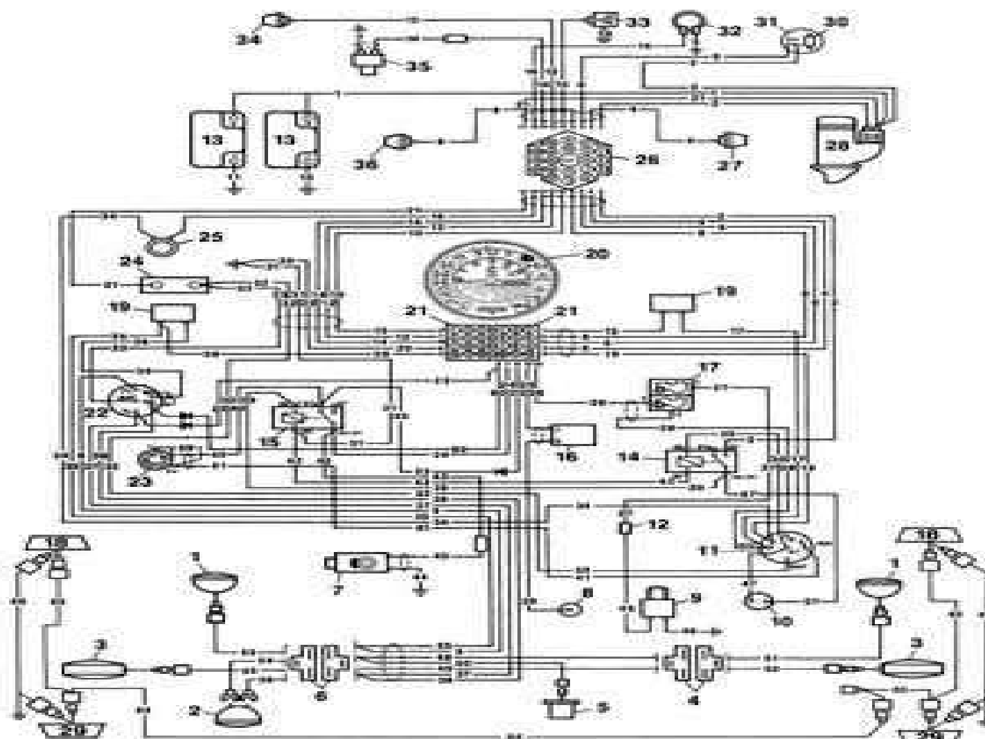
Fig. 1 — Wiring Diagram
