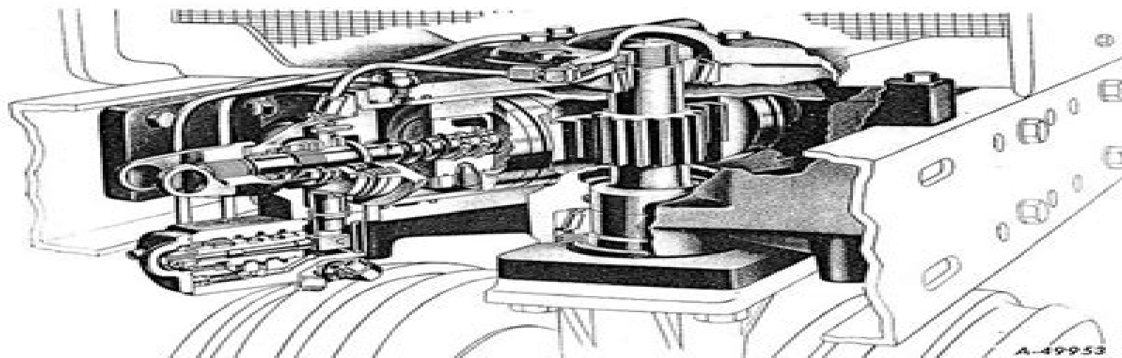
Illustr. 9. Cut-away view of the steering mechanism of a Ford 460 tractor.
