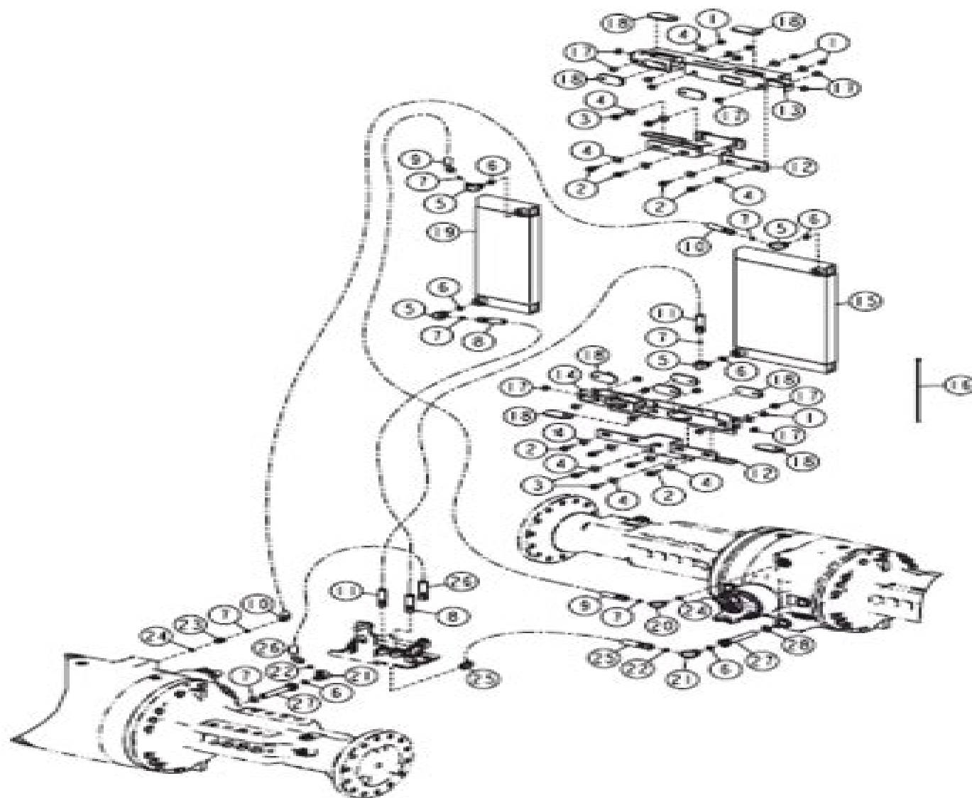
Axle Oil Cooler—Exploded View
