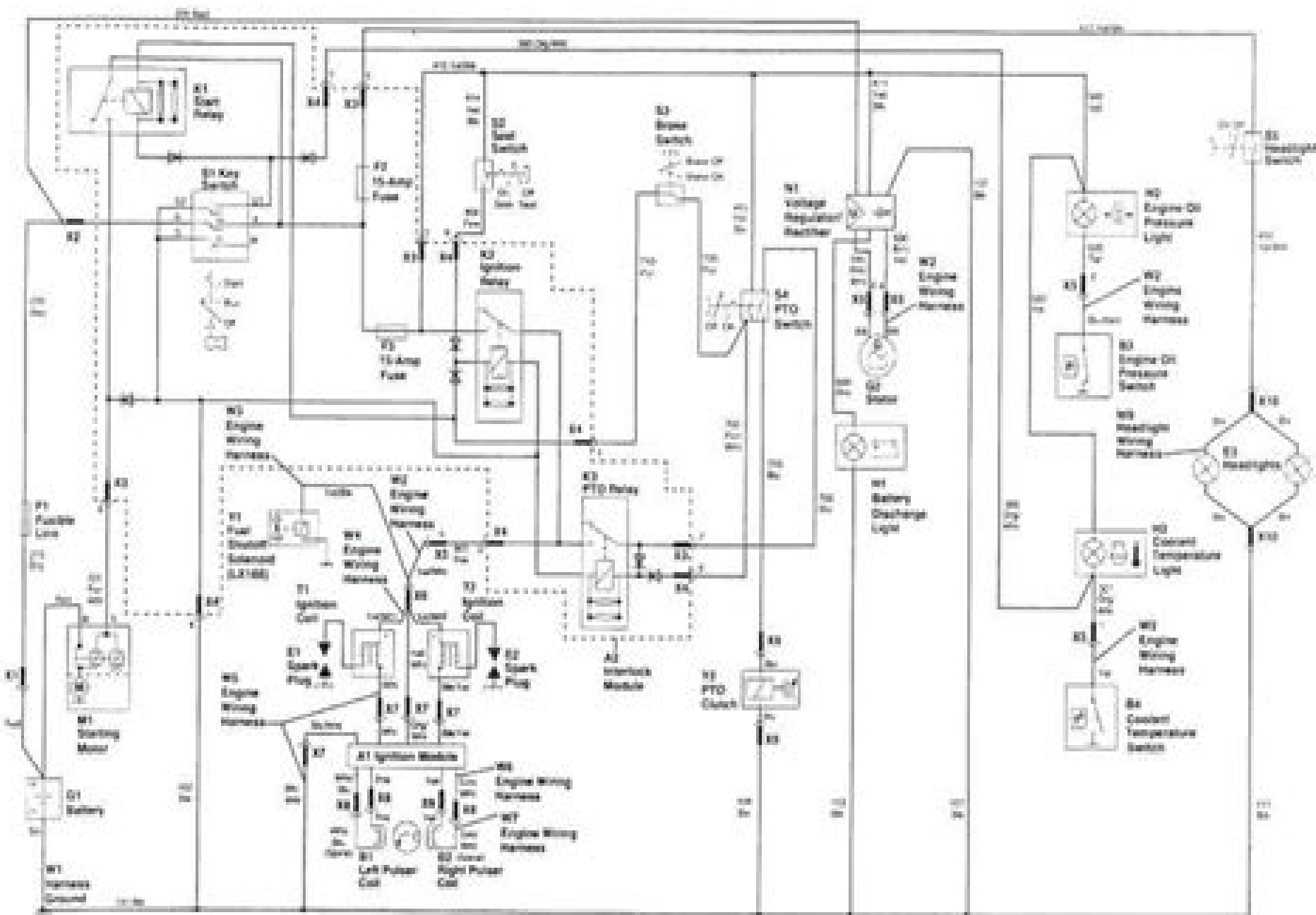
Fig. JD2-20-Wiring schematic for Models LX178 and LX188.
