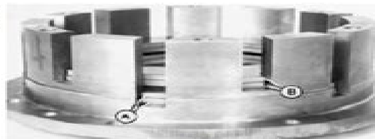
Drive Plates Installation
