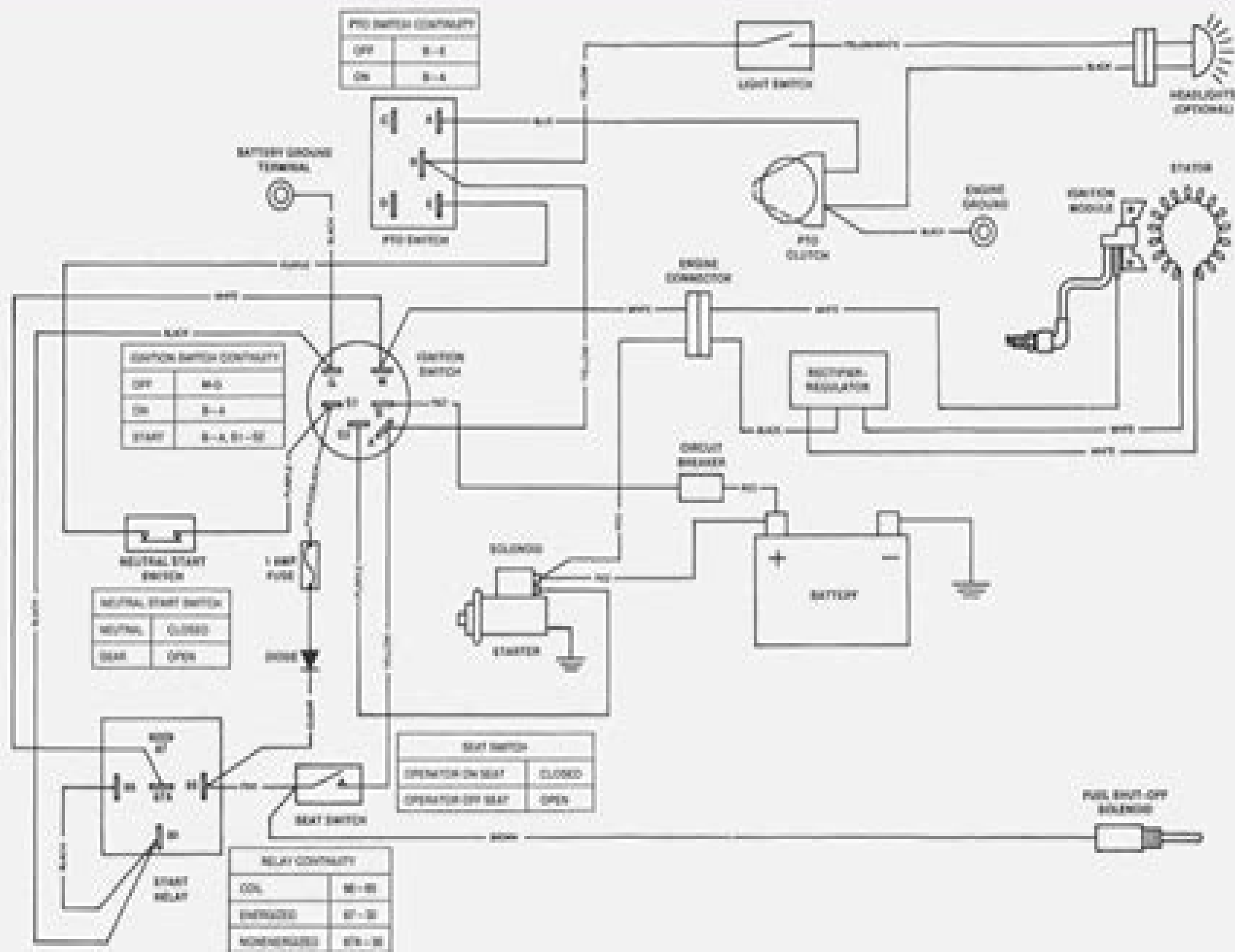
Fig. JD1-10-Wiring schematic typical of all models.
