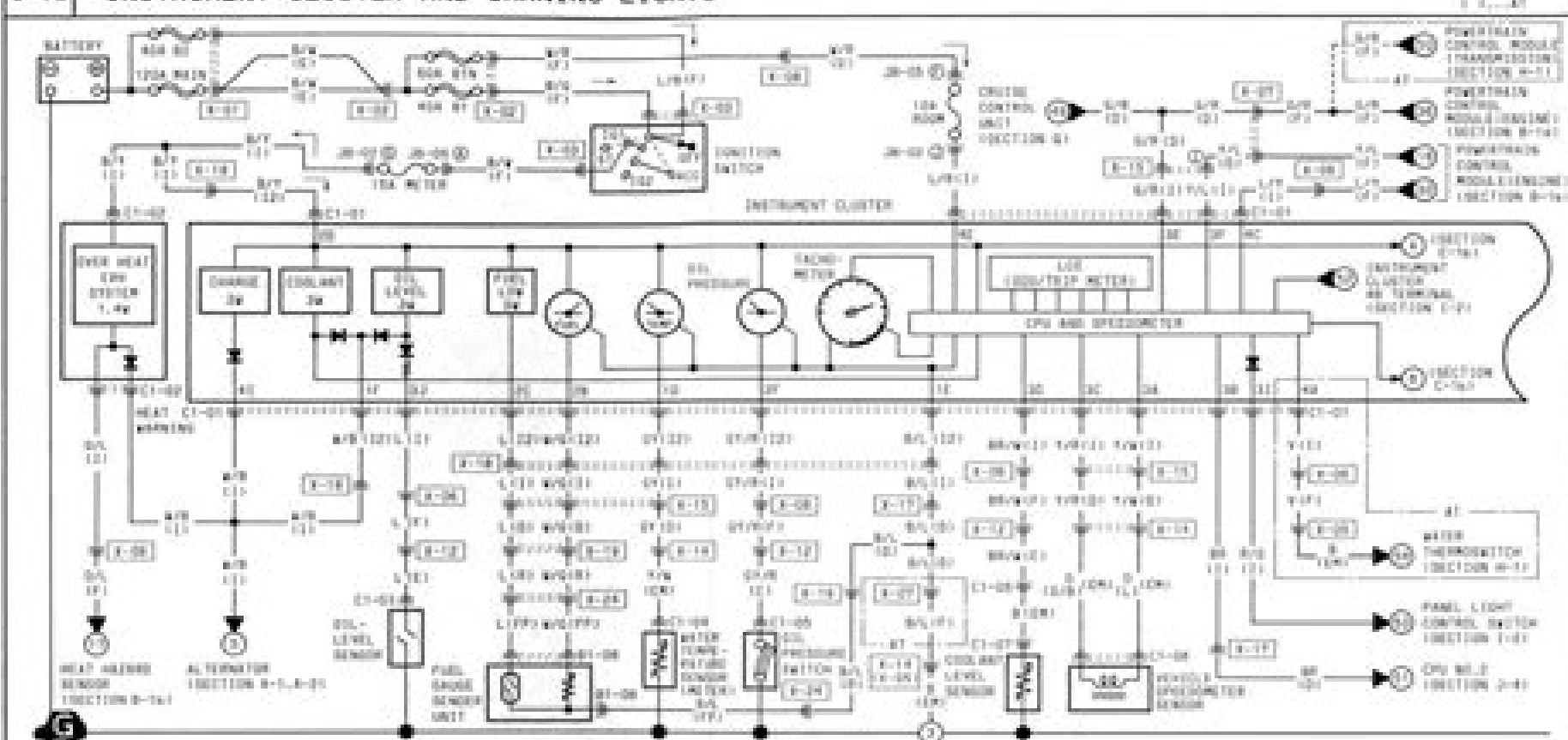
C1-01 INSTRUMENT CLUSTER
