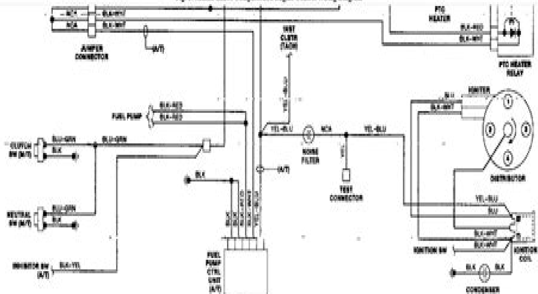
Fig. 1: Mazda B2300 Computerized Engine Control Wiring Diagram
