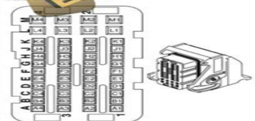
A6-605-LIN: End View
