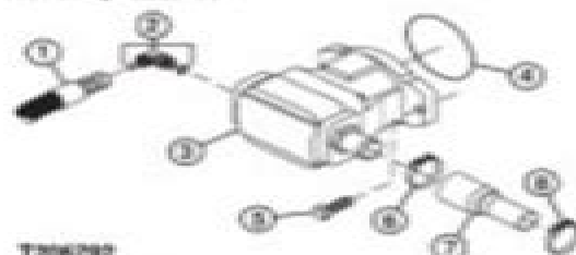
T2067902 Hydraulic Pump
