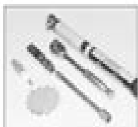
15.16 Tools required for spark plug removal, gap adjustment and refitting.
