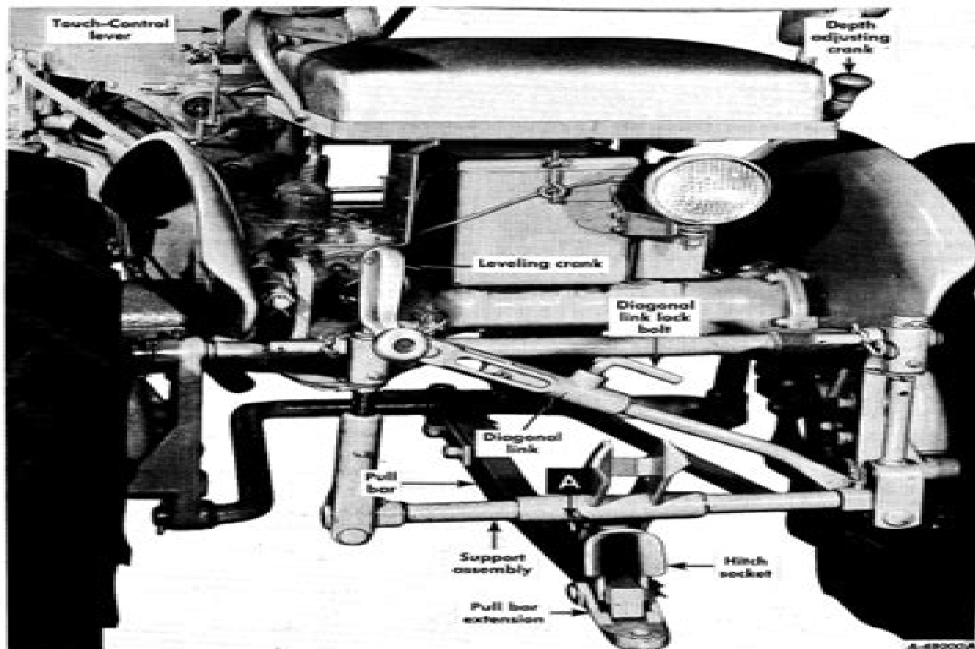
Illustr. 15 Rear view of Farmall Cub Tractor with Fast-Hitch.
