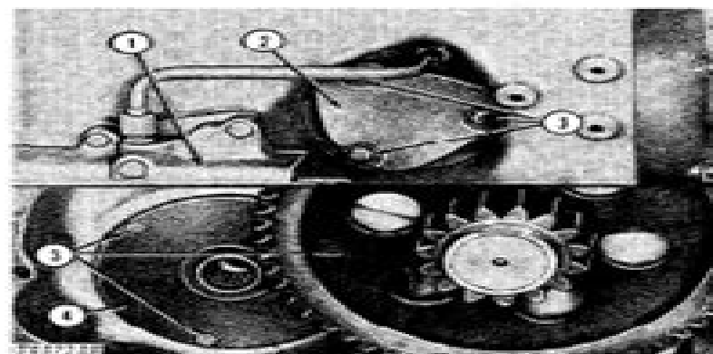
1—Winch Control Valve 2—Retainer 3—Cap Screws 4—Left Bearing Quill
