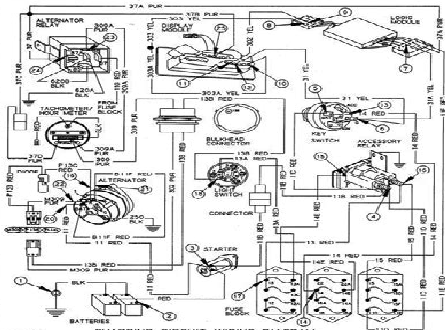
CHARGING CIRCUIT WIRING DIAGRAM (S.N. 766922-772238)
