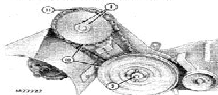
Fig. 20-Removing Chain, Sprockets and Sheave Assembly
