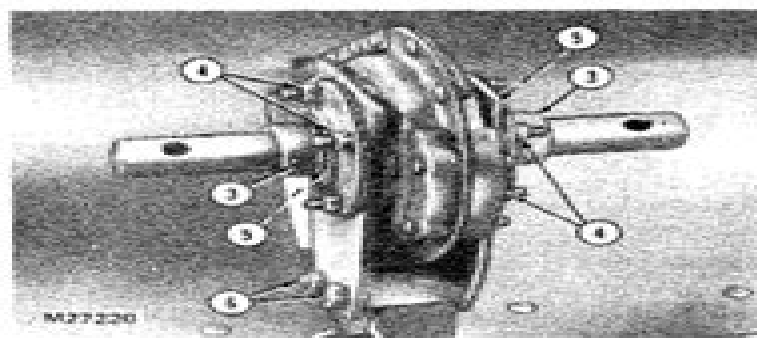
Fig. 18-Removing Locking Collars, Flangettes, Bearings and Plates
