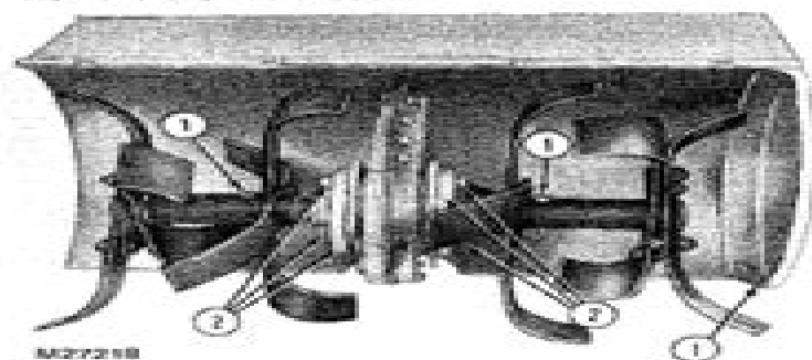
Fig. 17-Removing Shroud End Covers, Tines and Bearing Caps
