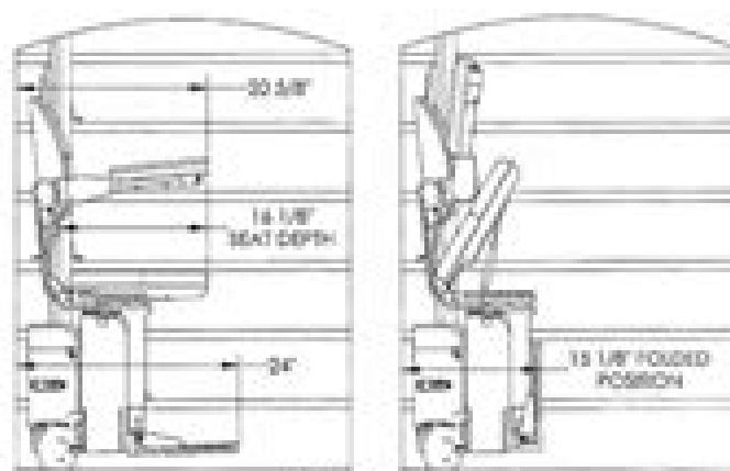
SIDE VIEWS
