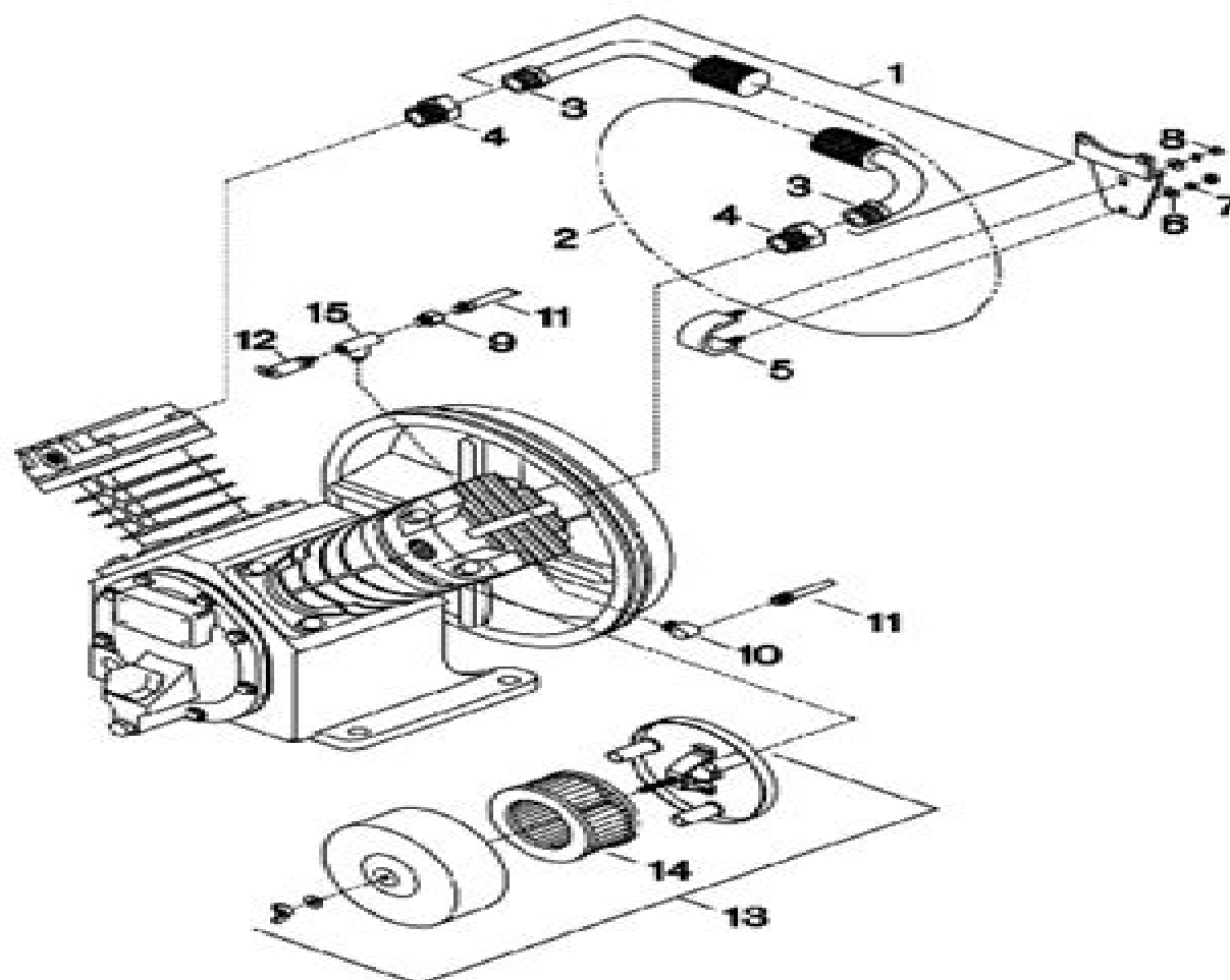
FIGURE 8. TYPICAL MODEL 347-B INTERCOOLER ASSEMBLY.
