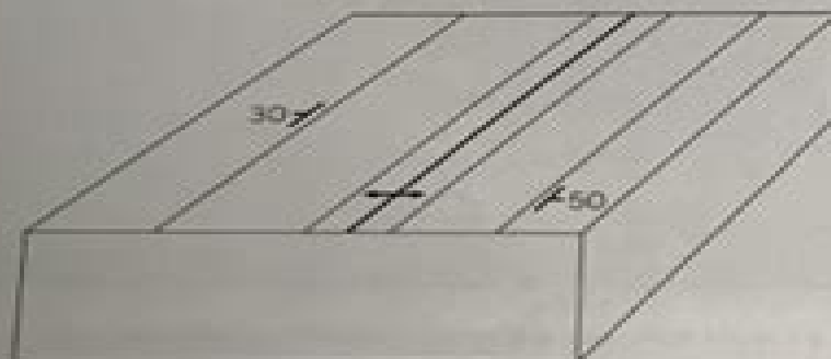
E. Complete the sides of the diagram. What geologic structure is this?
