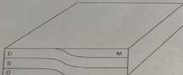
C. Complete top and side. Add appropriate symbols from Fig. 10.4. What type of fold is this?
