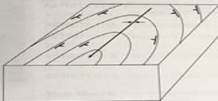
F. Complete the sides of the diagram. What geologic structure is this?
