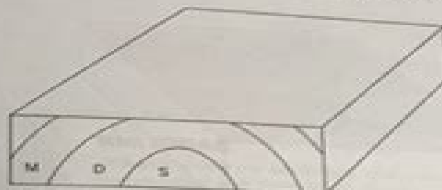
B. Complete top and side. Add appropriate symbols from Fig. 10.4. What type of fold is this?
