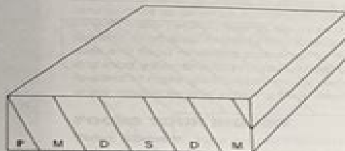
D. Complete top of diagram. Add appropriate symbols from Fig. 10.4. What geologic structure is this?
