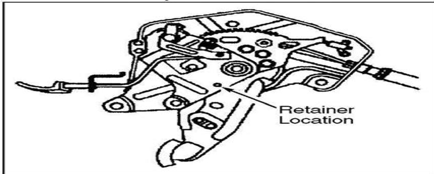
Fig. 14: Relieving Tension On Park Brake System Courtesy of FORD MOTOR CO.
