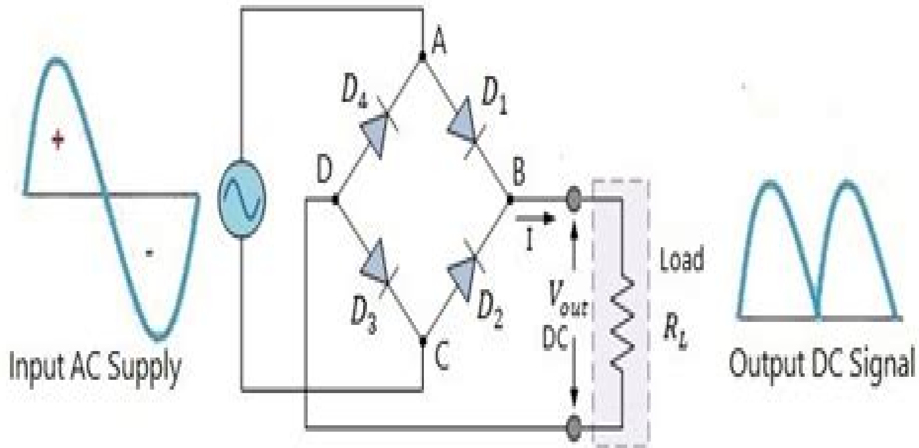
Full Wave Bridge Rectifier Circuit Diagram
