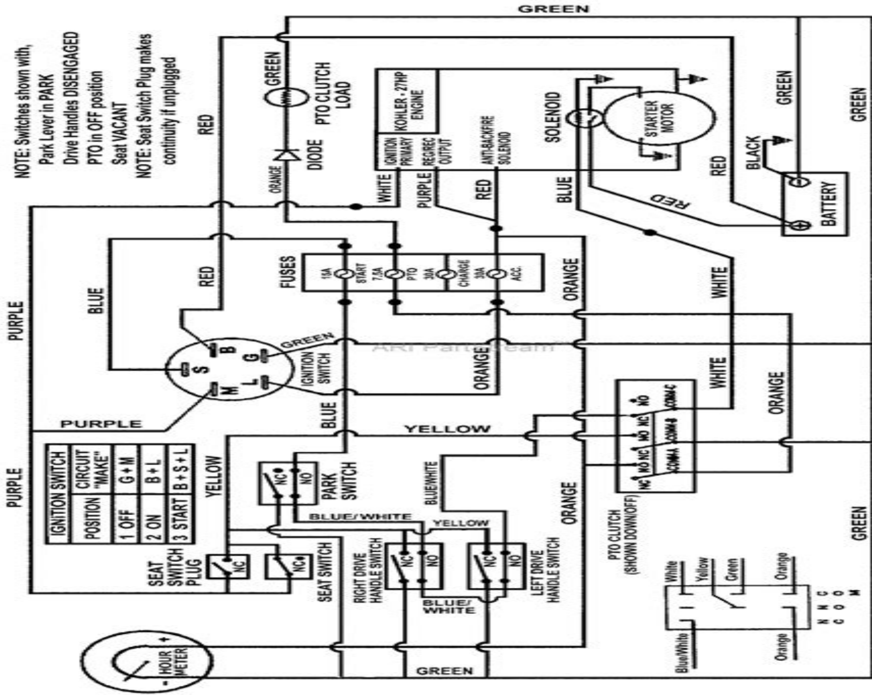
SCHEMATIC - WIRING HARNESS P.N. 29337
