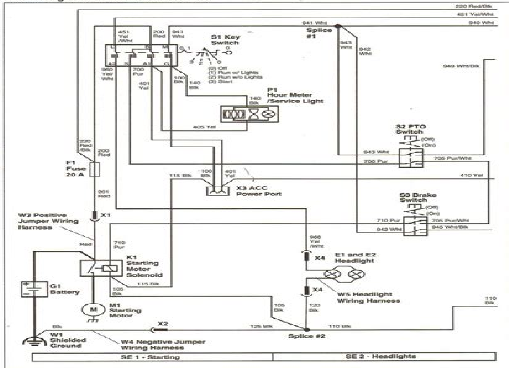
Main Wiring Schematic L100/L110/L120
