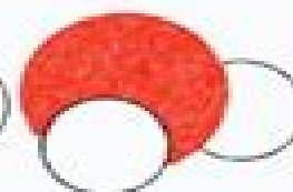
WATER ( H_2O )
