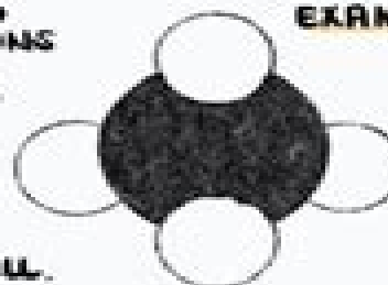
METHANE ( CH_4 )
