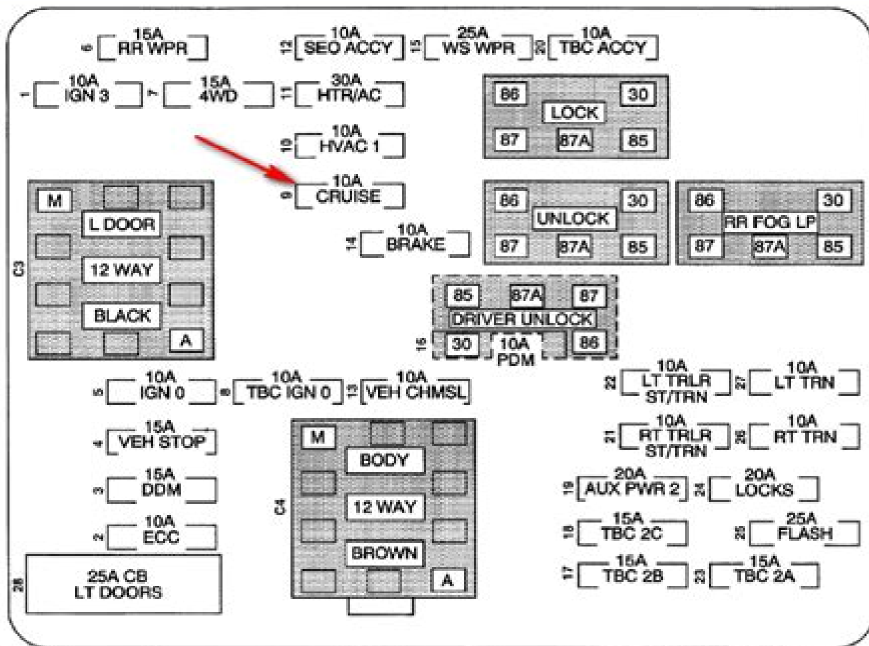
Fig. 2 Identifying Left Instrument Panel Fuse Block Components GENERAL MOTORS CORP.
