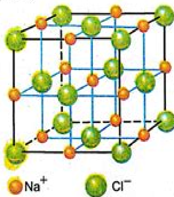
Figure 4.3 Regular arrangement of \text{Na}^+ and \text{Cl}^- ions in solid crystal of NaCl
