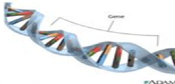
Figure 1. A short strand of DNA. The translucent bars on either side are the sugar-phosphate "backbone" of the molecule. The "rungs" of the twisted "ladder" are the nucleotide bases. Each "rung" is formed by either (T) hydrogen-bonded to adenine (A) or guanine (G) hydrogen-bonded to cytosine (C).
