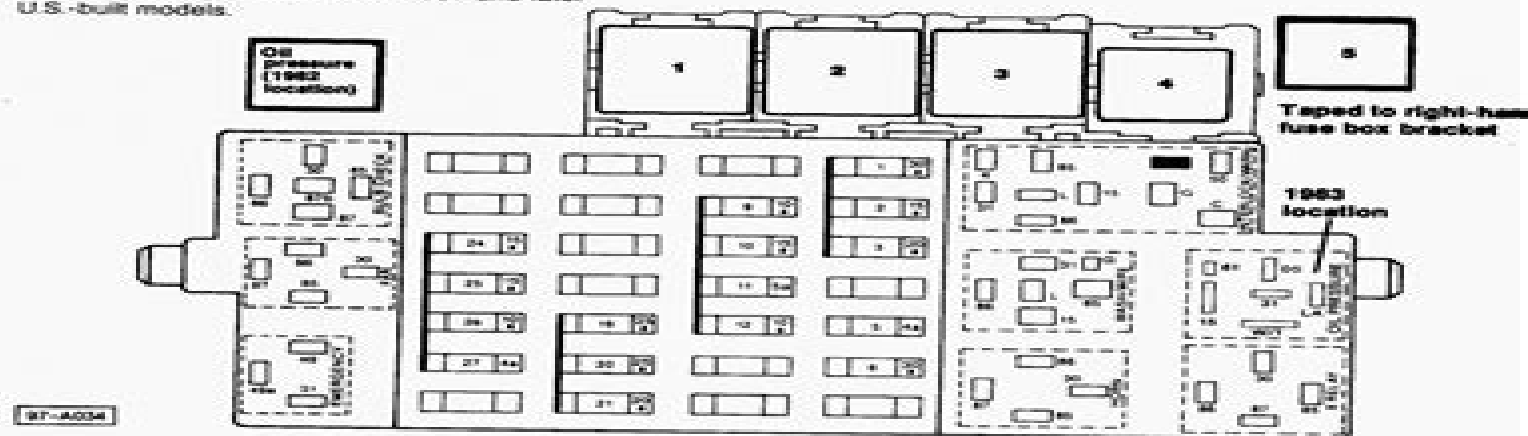
Fig. 13-3. Fuses and relays identified for 1981 and later U.S.-built models.
