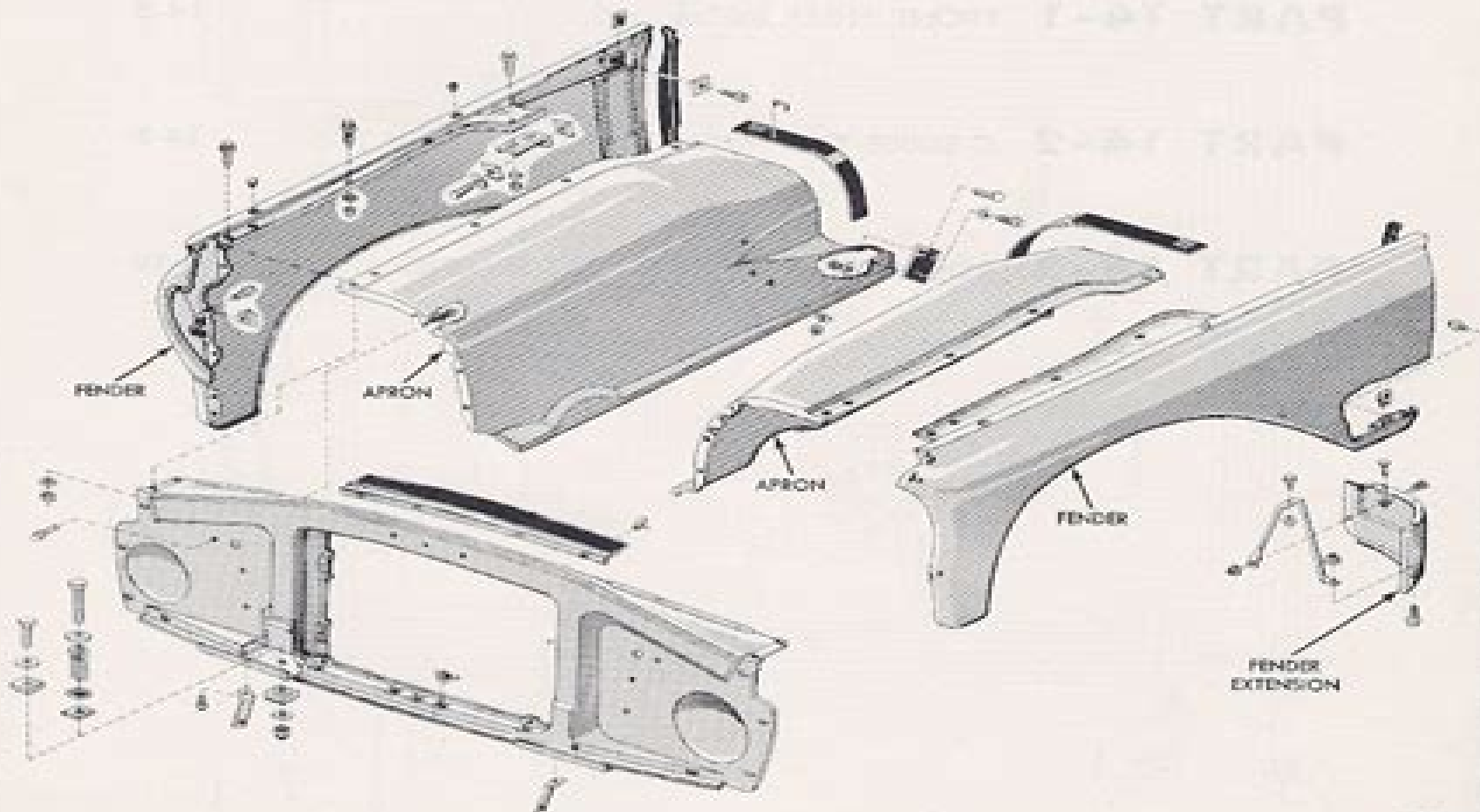
FIG. 1—Front Fenders—F-100 through F-700 and B-Series
