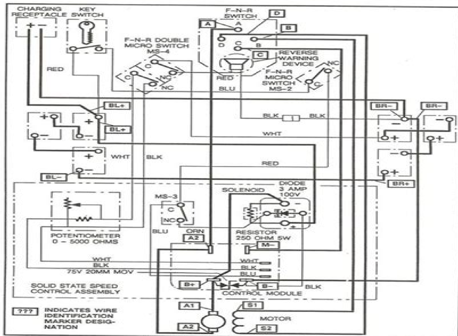
FIG. N-3 POWER WIRING DIAGRAM
