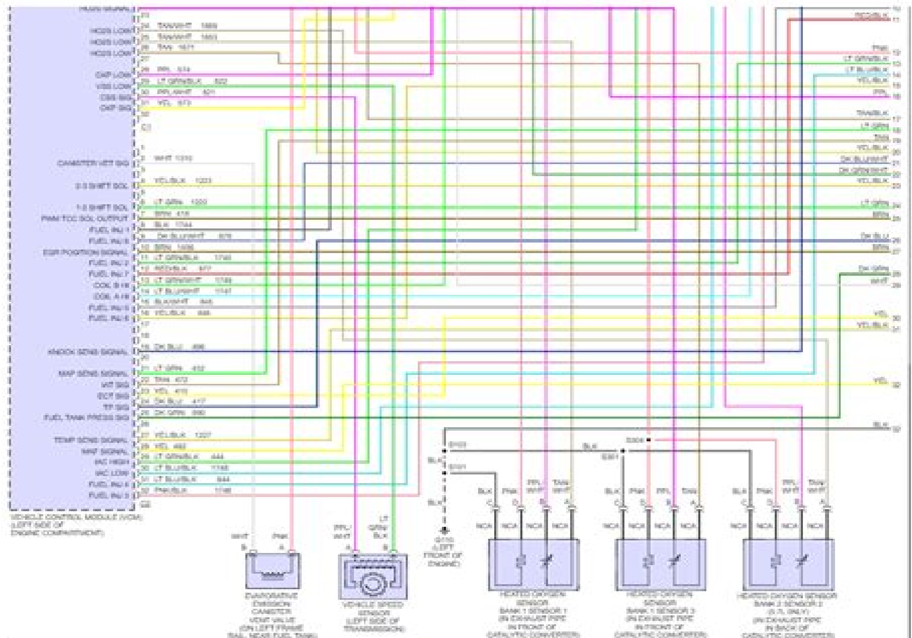
Fig 1: 5.7L VIN R, Engine Performance Circuits (1 of 4)
