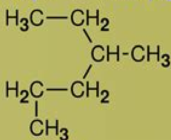
3-methylhexane
