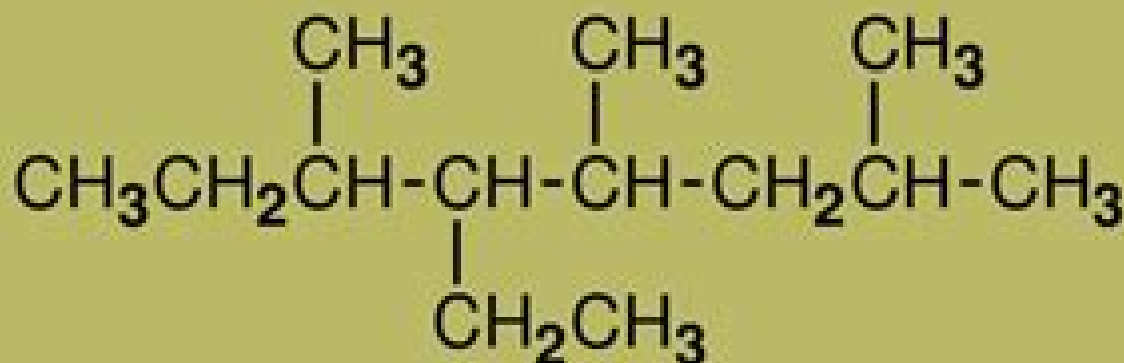
5-ethyl-2,4,6-trimethyloctane
