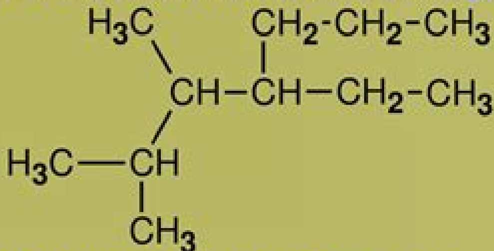
4-ethyl-2,3-dimethylheptane
