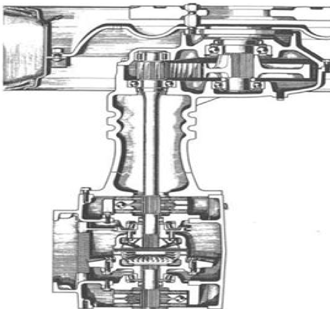
Fig. 1 - Cross-Section: Rear Axle, Differential, Brakes and Final Drives.
