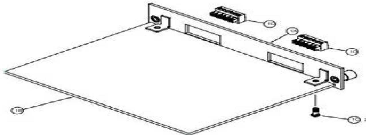
Figure 6-m: Dual Analog Output Assembly
