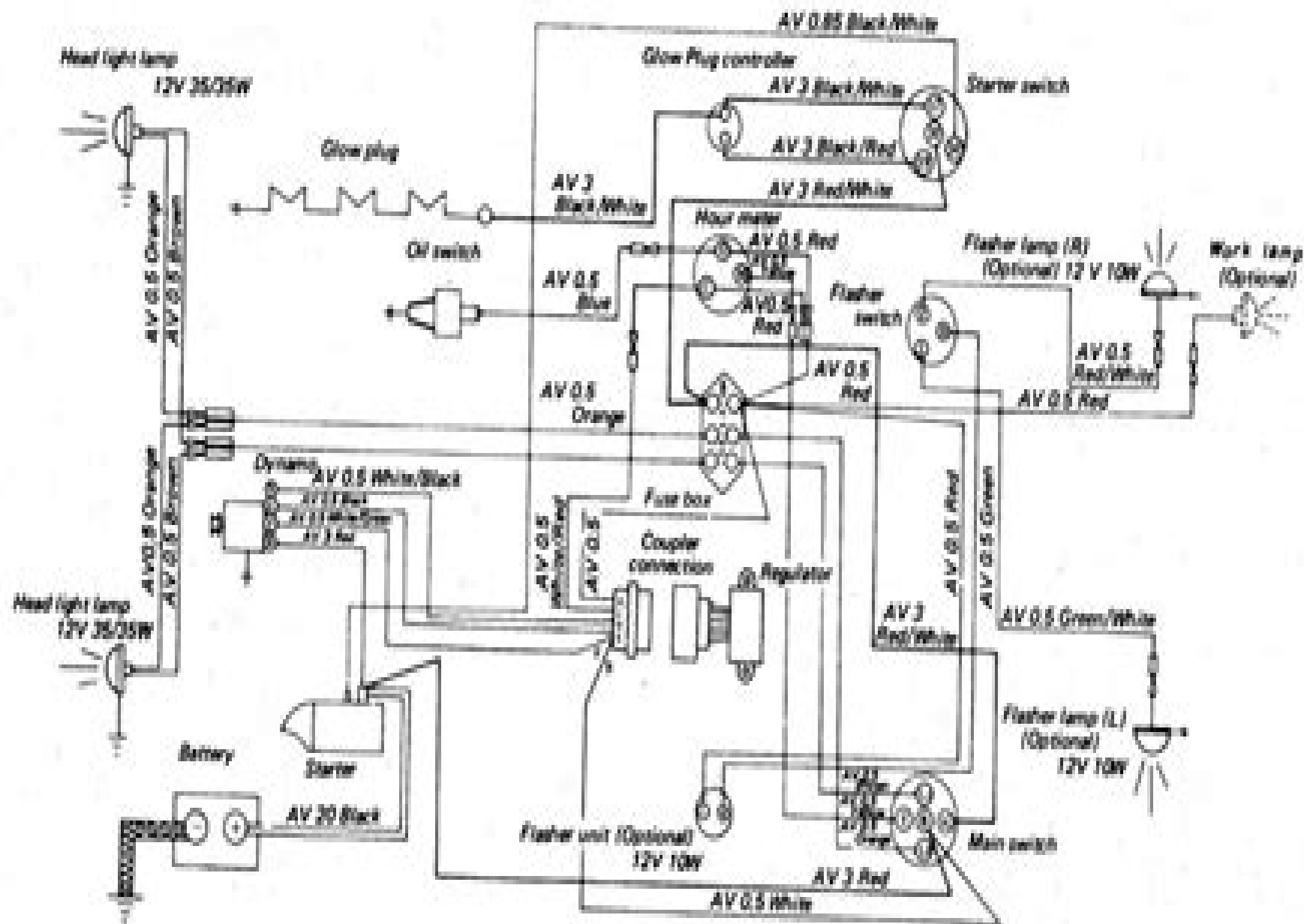
Fig. 153 – Schematic wiring diagram for Models L225 and L225DT.
