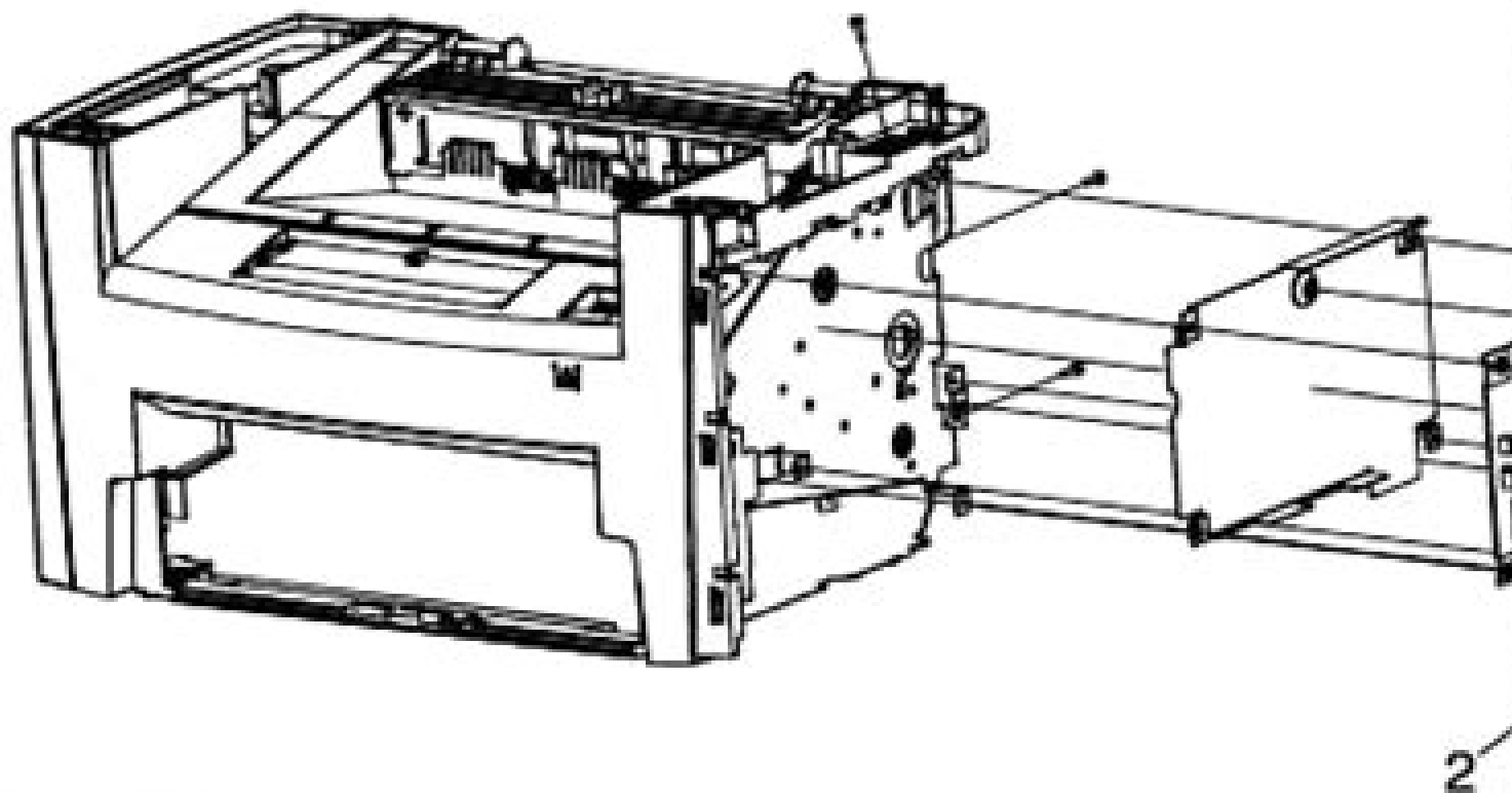
Figure 7-19 Formatter and LIU
