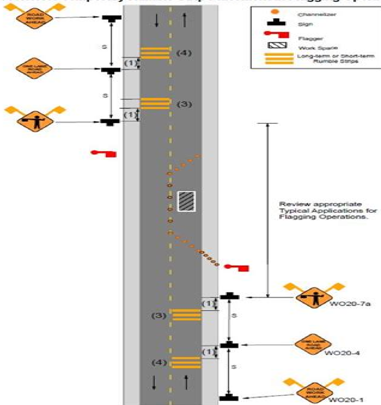
Figure: 616.6.87.1 Temporary Rumble Strip Placement in Flagging Operations
