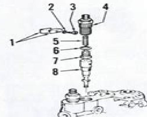
Fig. 15—Exploded view of fuel delivery valve. Remove No. 1 fuel delivery valve to spill time engine.
