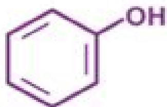
Phenol
