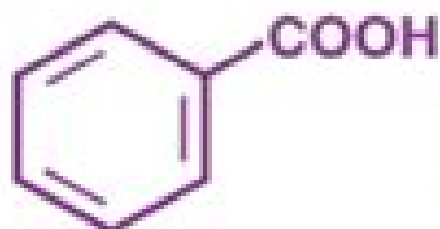
Benzoic acid
