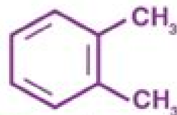
Ortho-xylene
