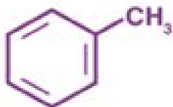
Toluene
