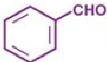
Benzaldehyde
