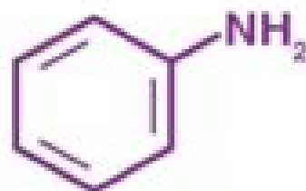
Aniline
