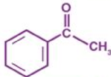
Acetophenone
