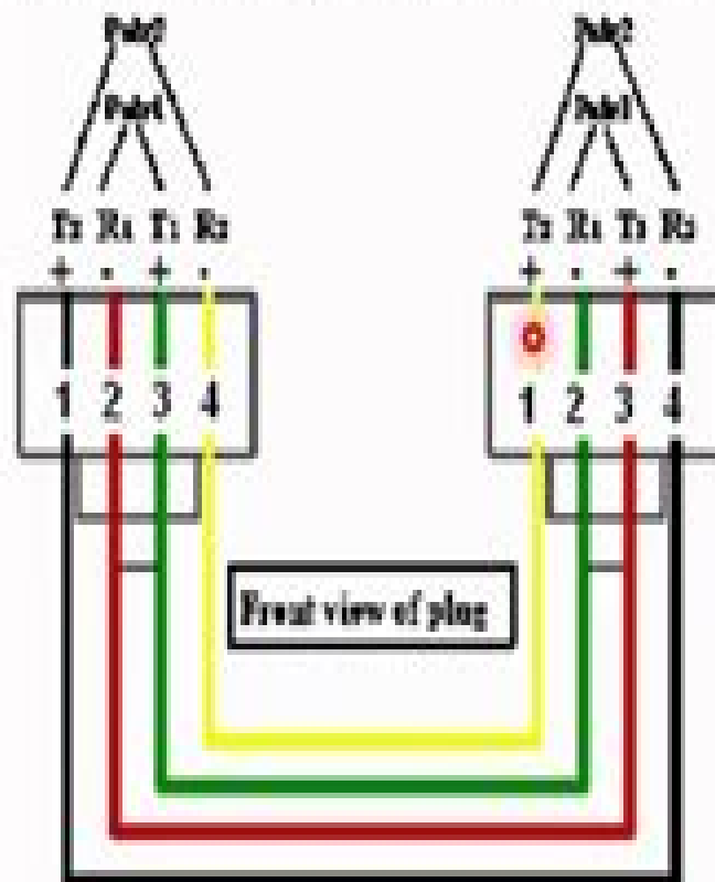
Both ends of a reversed wired phone cord
