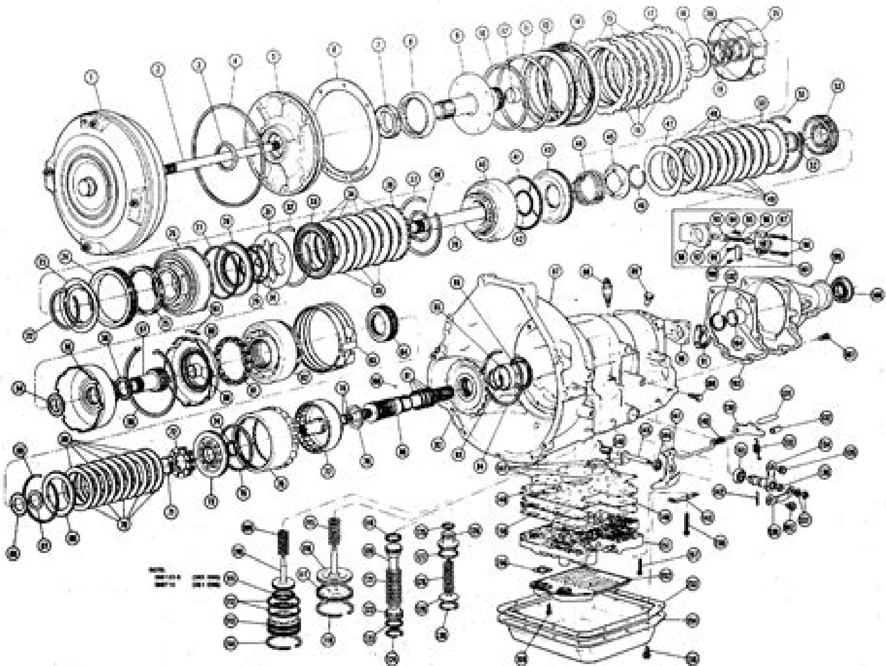
The Ranger Station - Exploded View Of A609 Transmission
