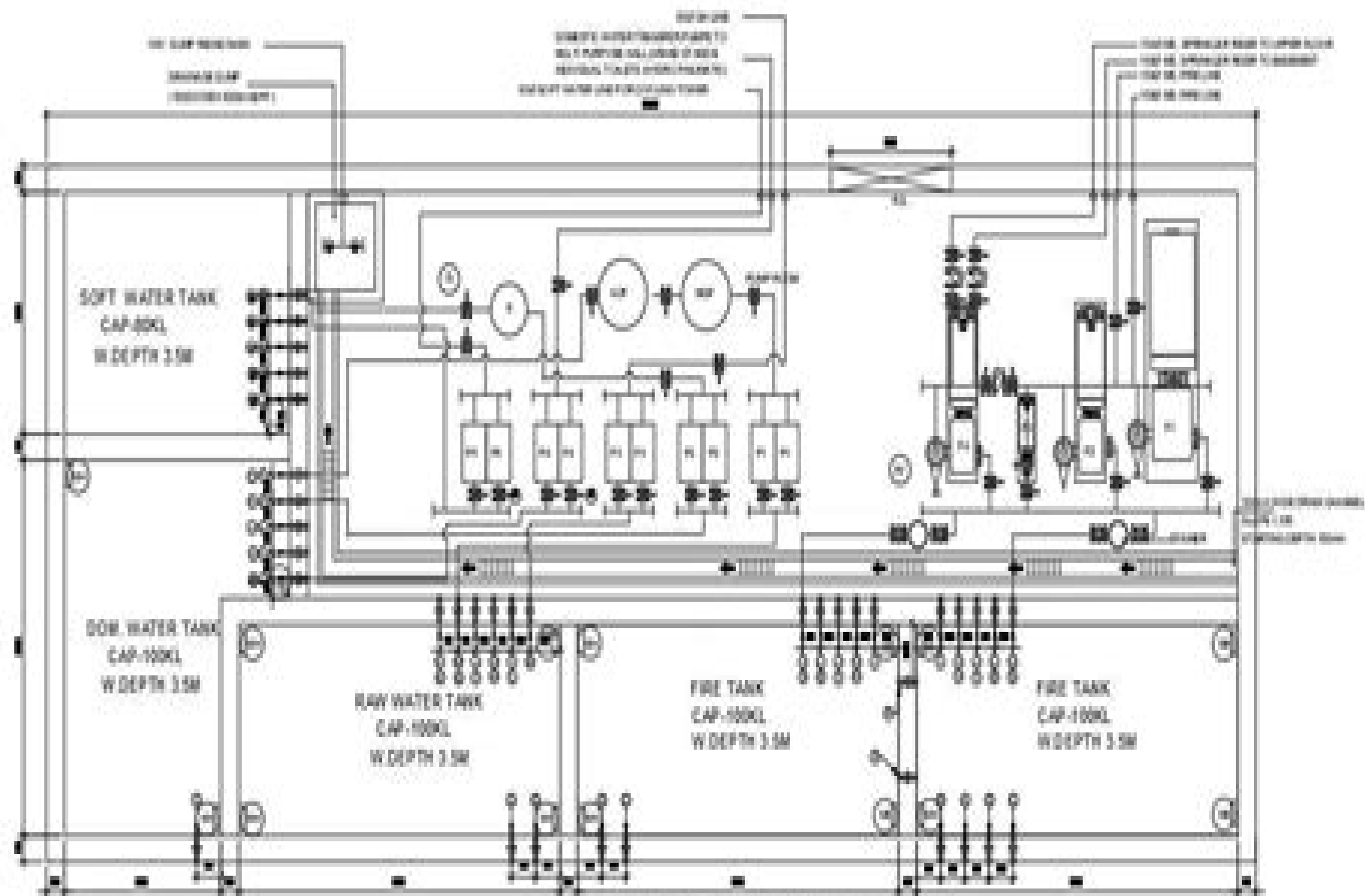
PUMP ROOM PIPING LAYOUT
