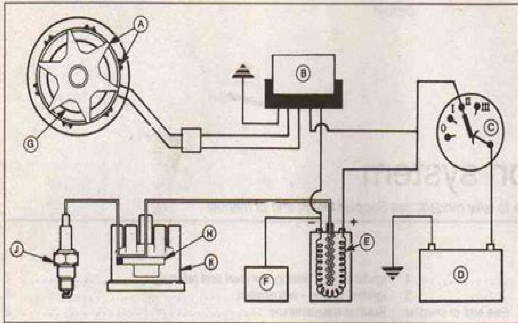
Fig. 4.1 Diagram of the breakerless ignition system (Sec 1)
