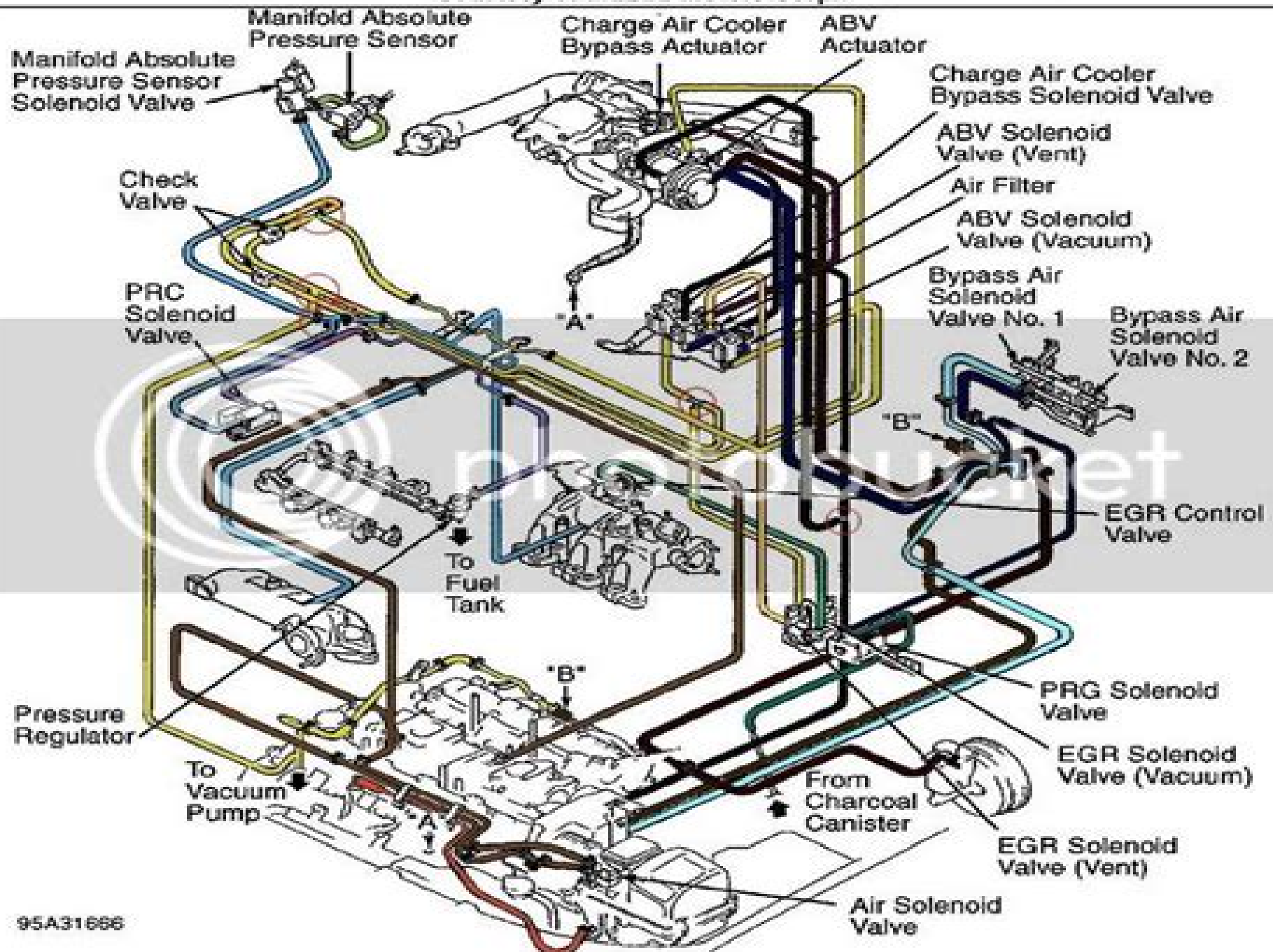
Fig. 2: Vacuum Diagram (Millenia S 2.3L) Vacuum Hose Routing Courtesy of Mazda Motors Corp.
