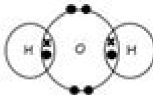
Water ( \text{H}_2\text{O} )
