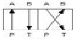
Spring Actuated
