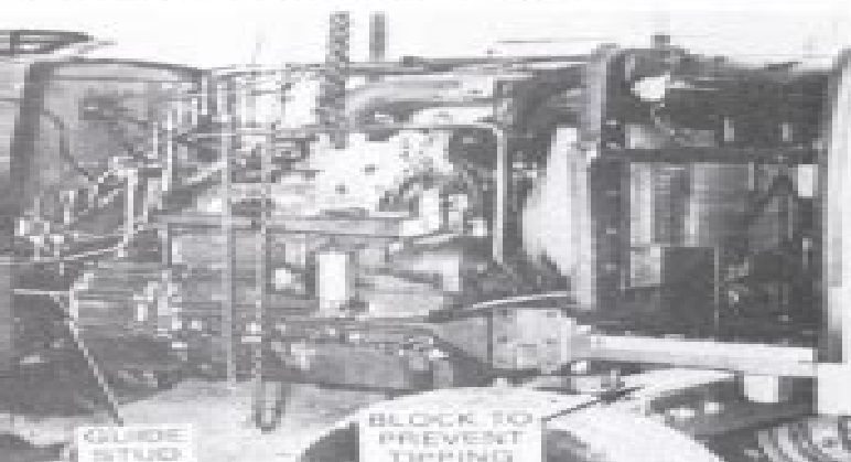
Fig. 127—View showing supports necessary when splitting. (See cylinder model to show front block used to substitute for left block.)
