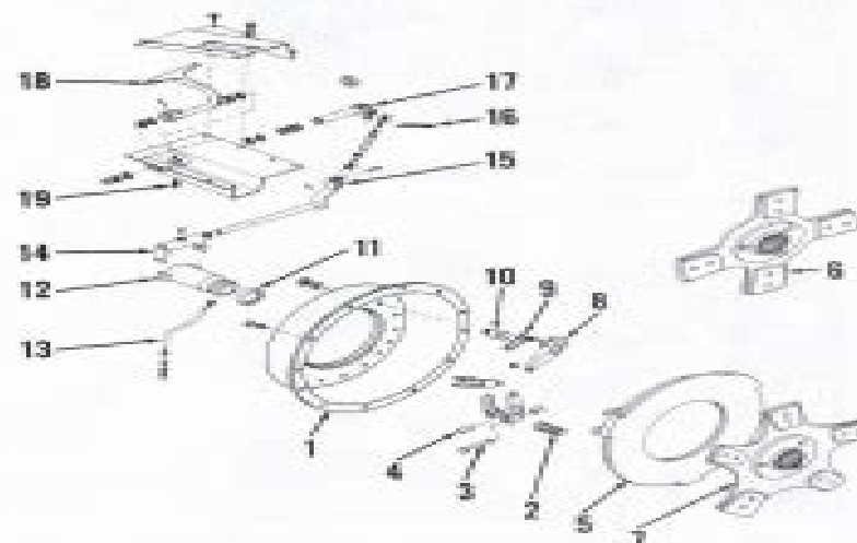
Fig. 198—Exploded view of clutch and linkage. Disc (5) with four pads is used with brown springs (2) on SAE 14005 models only.
