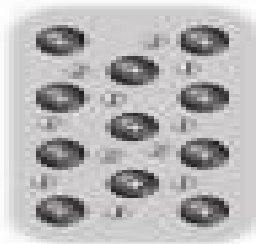
Group 1 Metal Atoms
