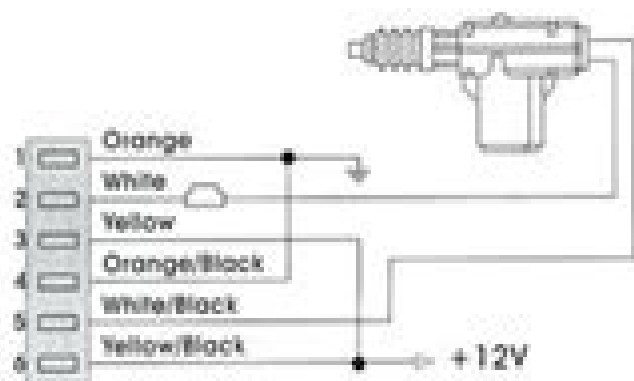
Positive/Negative trigger
